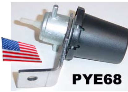
PYE68 .....DISTRIBUTOR VACUUM CONTROL VALVE The rare Vacuum Control Valve, #9773623. We only have a limited supply. Fits 1968 V8 w/ manual trans and 1969 RA III w/ manual trans.
